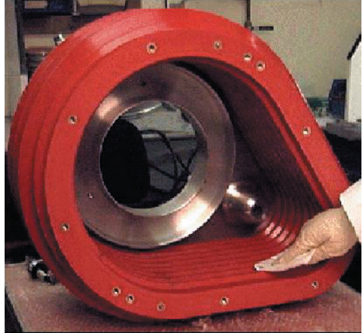
Accelerator Bushing for the Varian Viision Implanter
